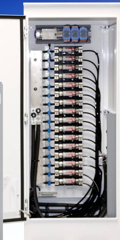
250kw-650kw Recombiner
