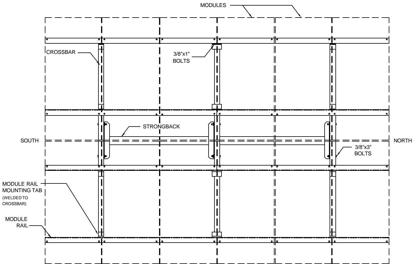
END VIEW
