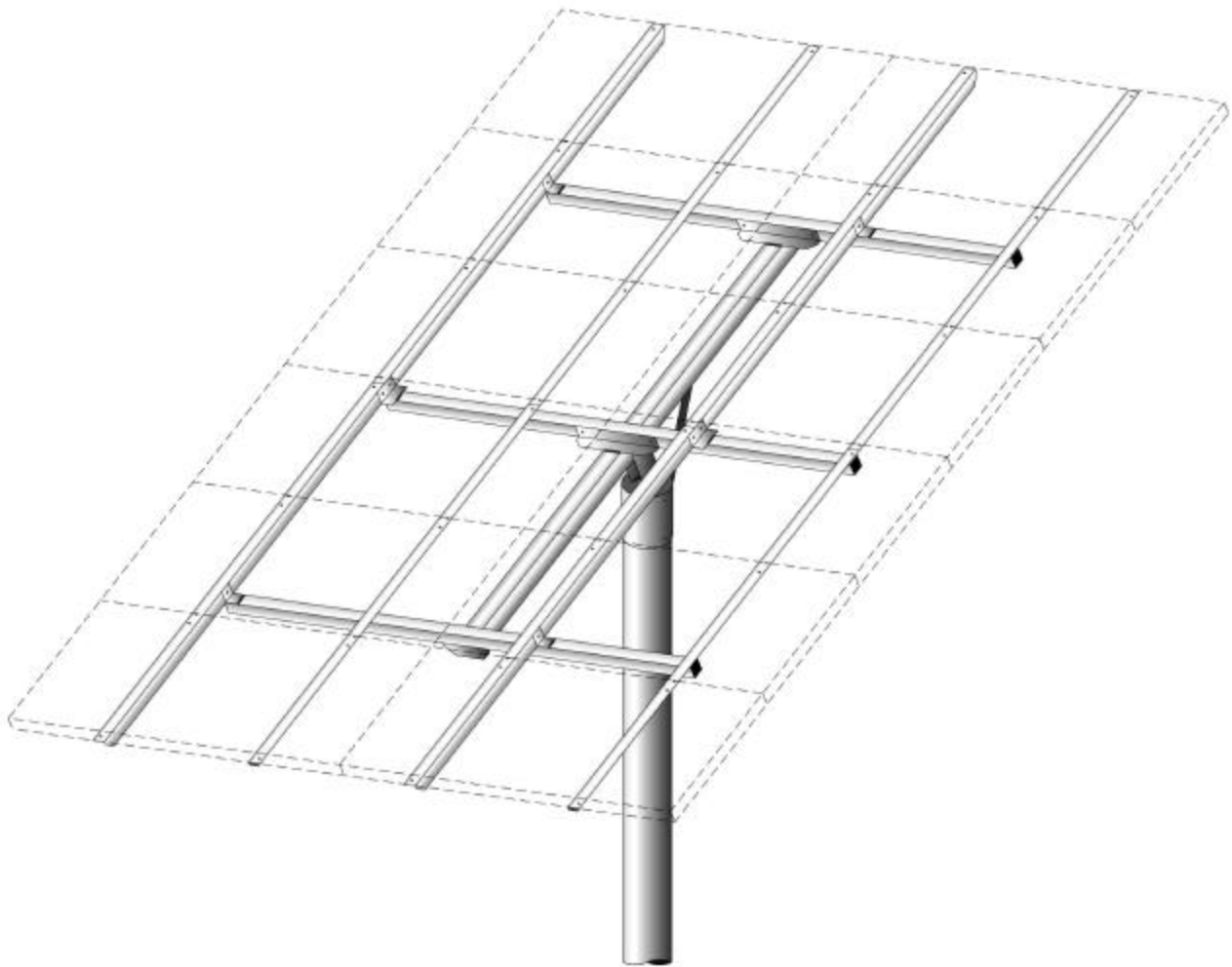
SERIES 120-6 Rack
