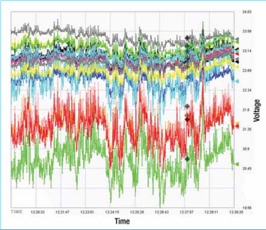
Figure 2. Voltage distribution of a typical crystalline PV string.
