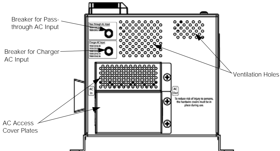
Figure 1-2 AC Side of the Xantrex TR Series
