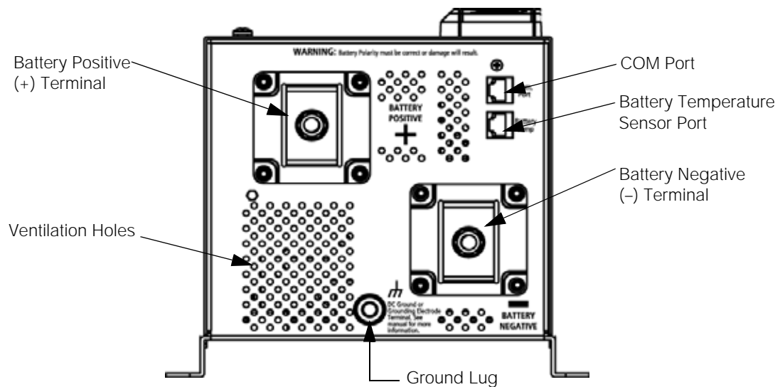
Figure 1-3 DC Side of the Xantrex TR Series
