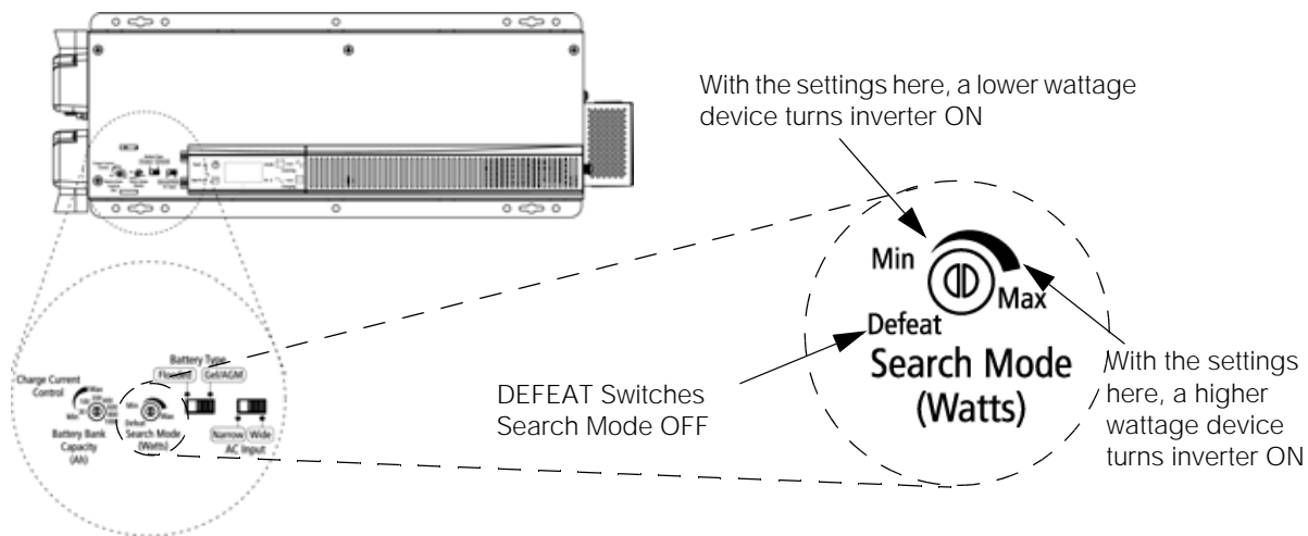
Figure 2-5 Search Mode Potentiometer Adjustment
