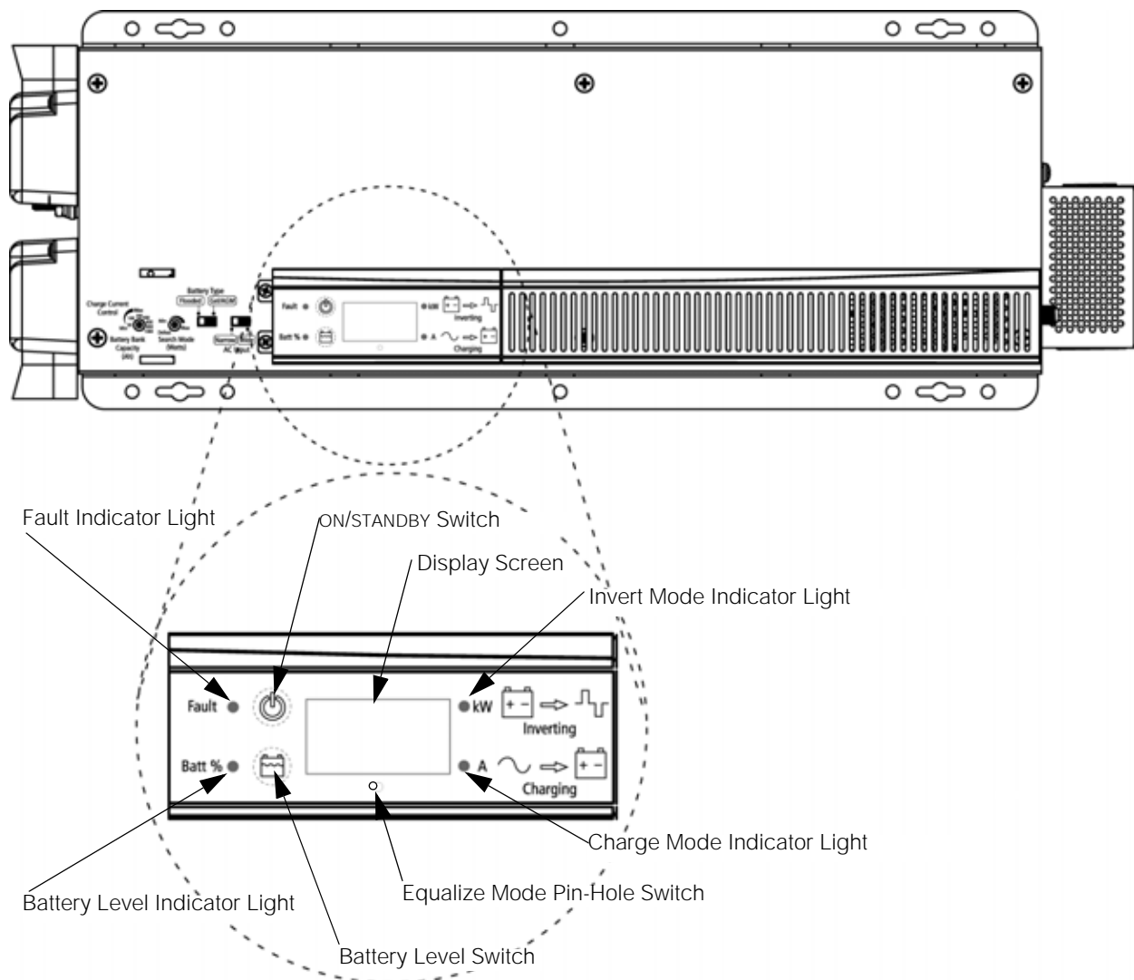
Figure 2-1 Front Panel User Interface
